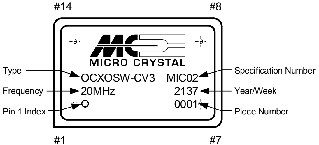
Laser marking OCXOS Package: (top view)
